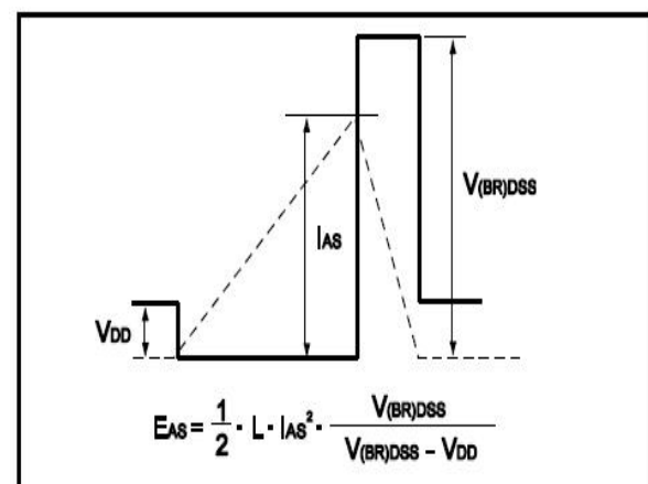
Fig.13 Avalanche Waveform
