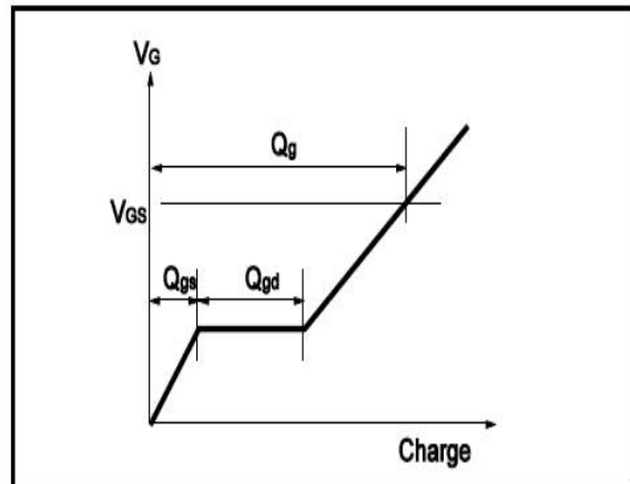
Fig.9 Gate Charge Waveform
