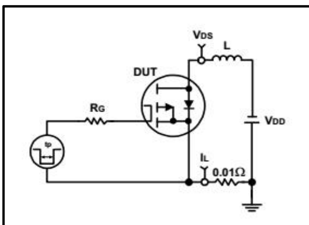
Fig.12 Avalanche Measurement Circuit
